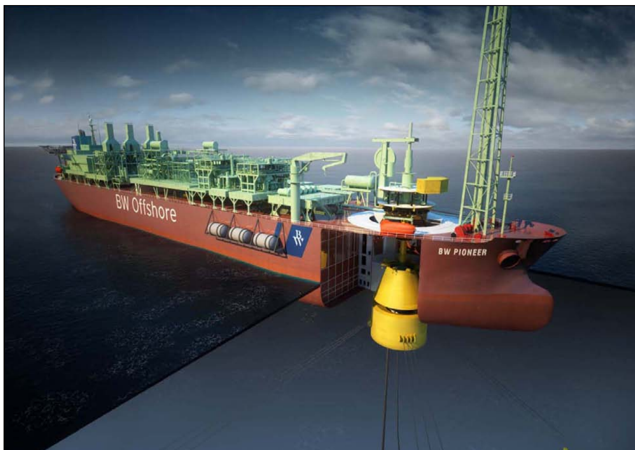
Figure 19. The BW Pioneer , the double-hulled tanker that will serve as the FPSO for the Cascade and Chinook developments. (Depiction courtesy of Petrobras.)
